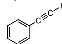
phenylacetylene
